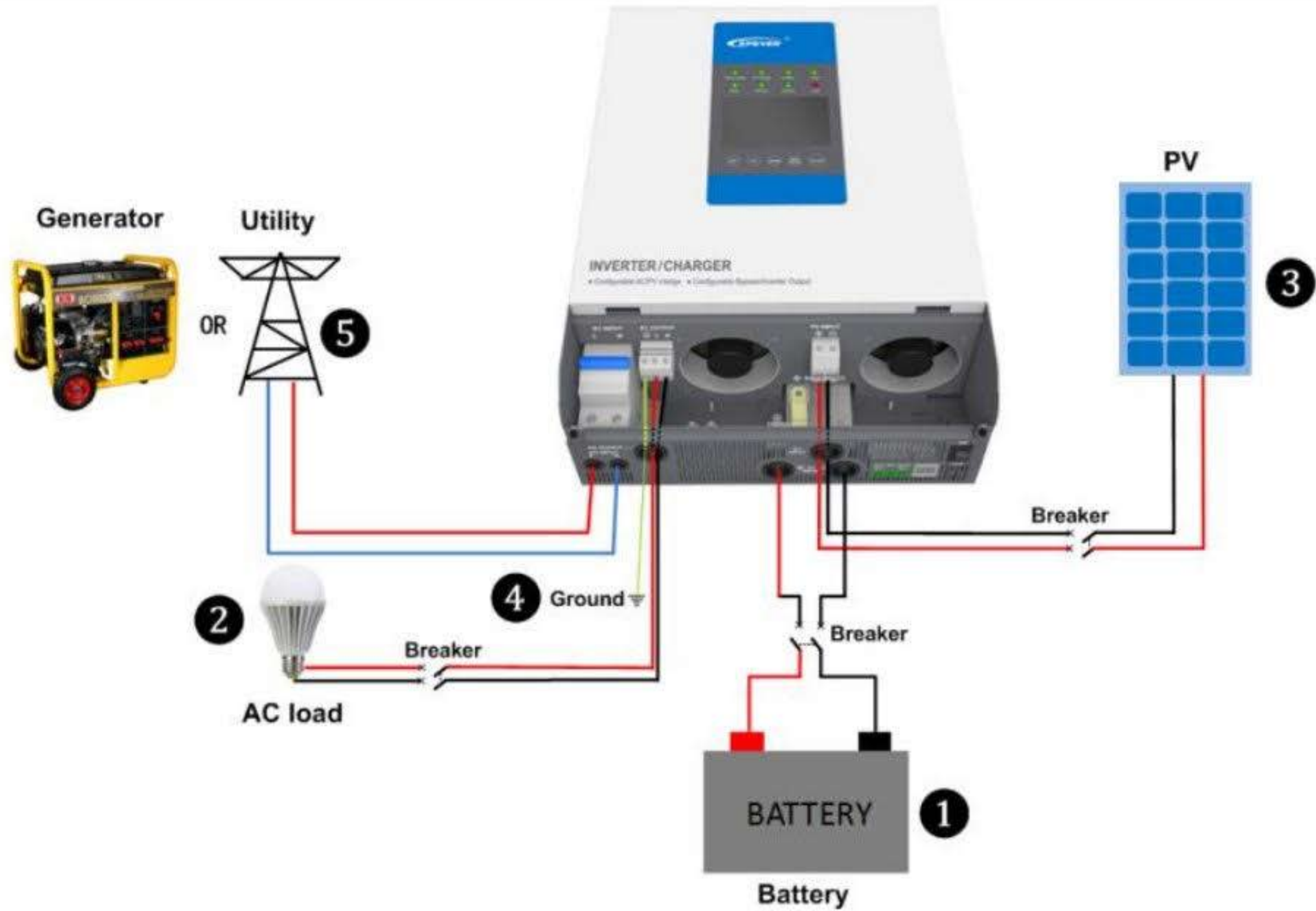
Figure 2-3Wring Diagram
